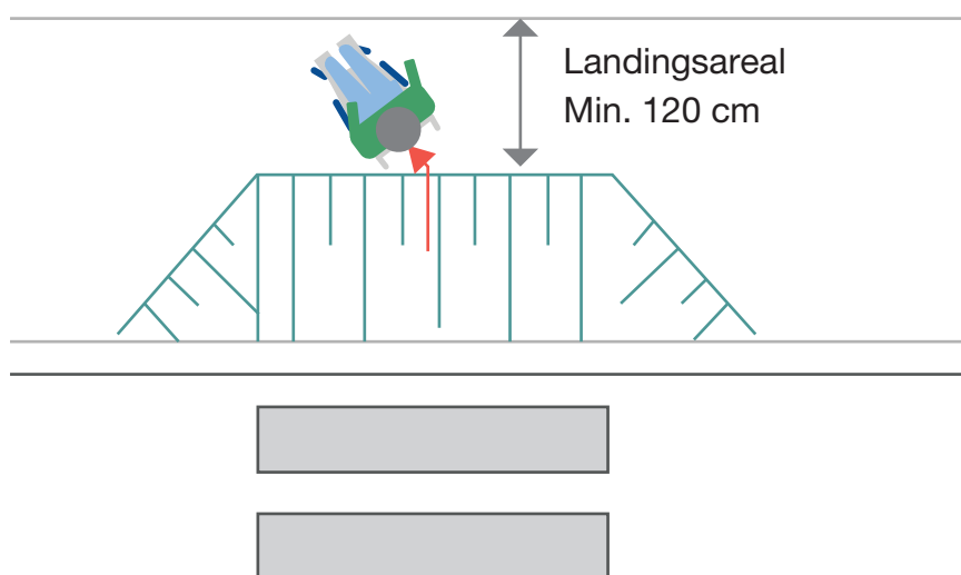
Figur 3-11: Figur viser landingsareal for rullestol.
